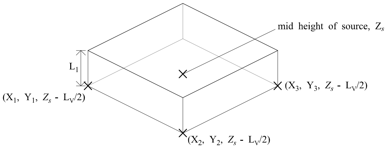
Figure 2 Definition of a volume source
