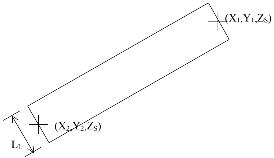
Figure 1 Definition of a line source
