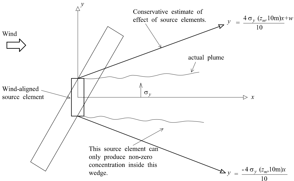
Figure 3 Domain of influence of source element. w is the half width of the wind aligned element.
