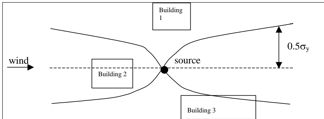
Figure 2. Example source and building configuration. Buildings 2 and 3 could be included in the effective building, but building 1 will not be included.
