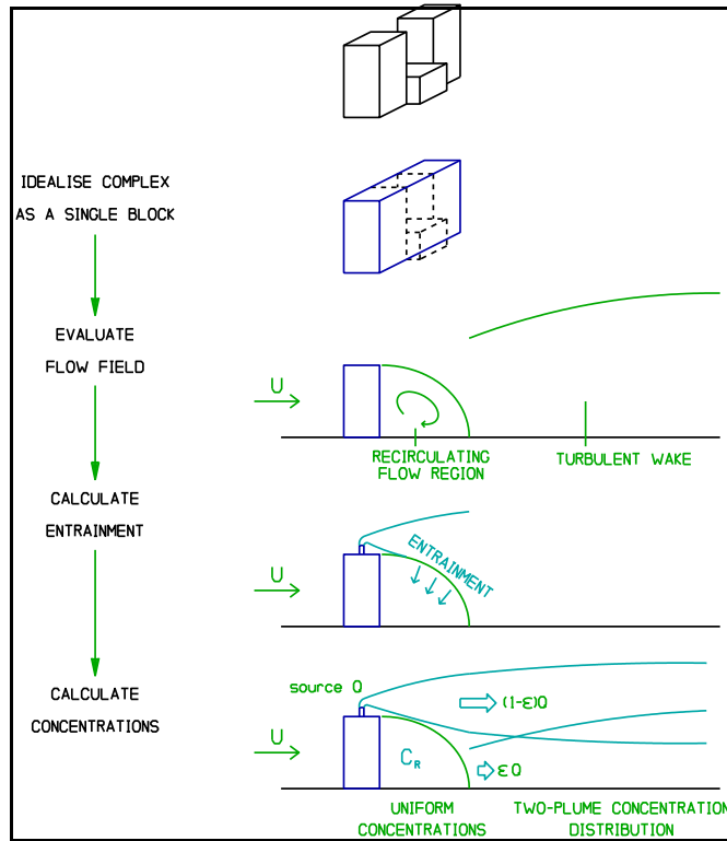
Figure 1.4 – Stages in the analysis of building effects.
