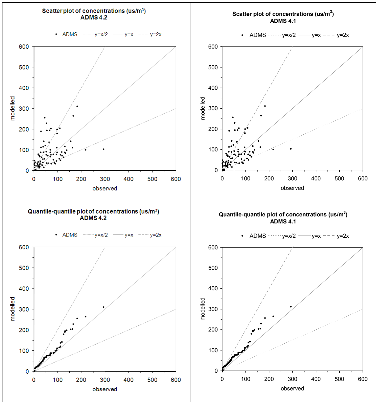
Figure 5 – Scatter plots and quantile-quantile plots of ADMS results against observed data ( \mu\text{g}/\text{m}^3 ).
