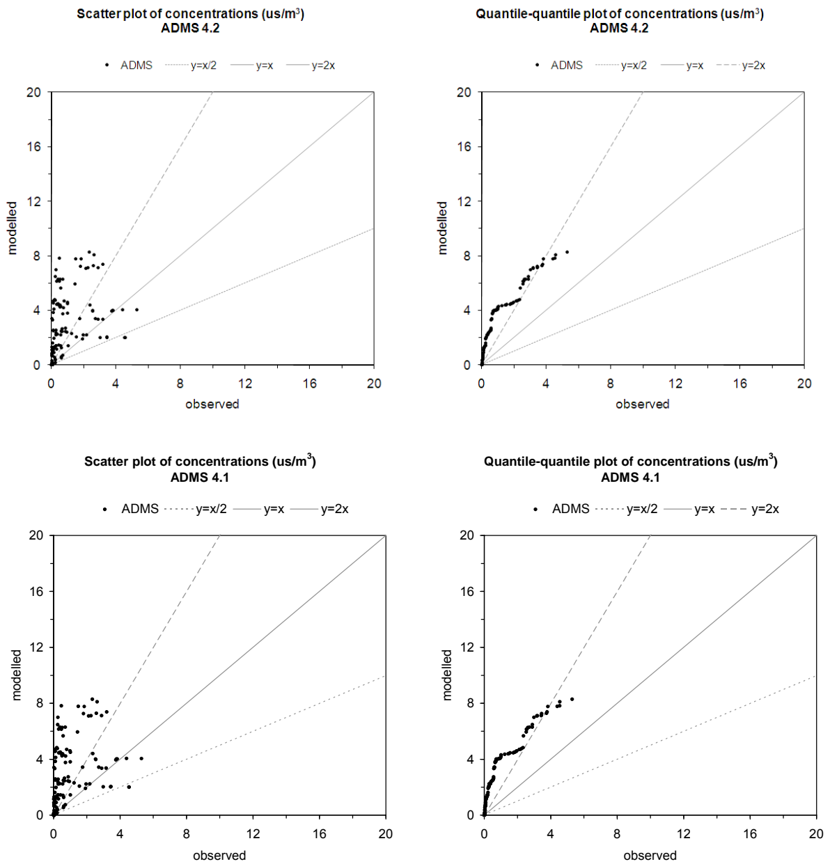
Figure 4 – Scatter plots and quantile-quantile plots of ADMS results against observed data (us/m 3 ).
