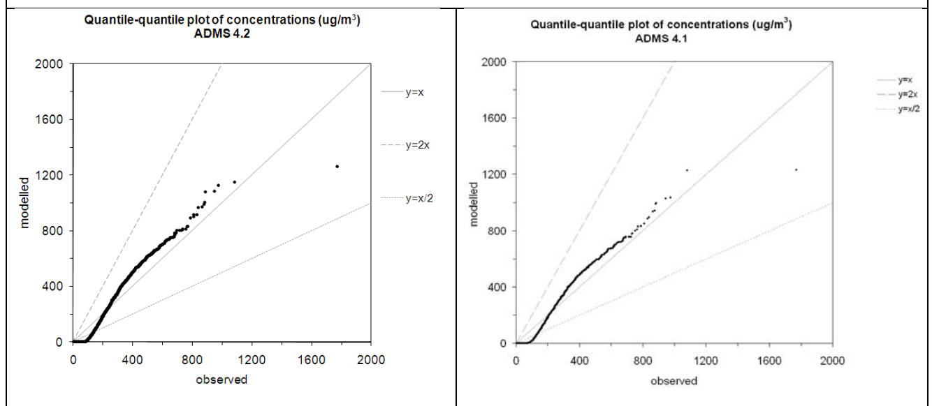
Figure 5 – Quantile-quantile plots of ADMS results against observed data for the ground-level receptors ( \mu\text{g}/\text{m}^3 ).
