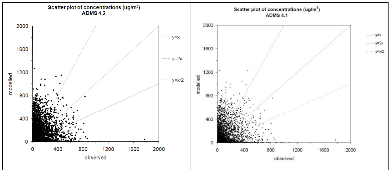
Figure 4 – Scatter plots of ADMS results against observed data for the ground-level receptors ( \mu\text{g}/\text{m}^3 ).
