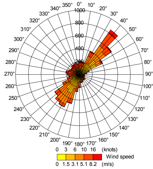
Figure 3 – Wind rose.
