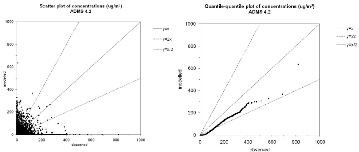
Figure 5 – Scatter plots and quantile-quantile plots of ADMS results against observed concentrations (ug/m 3 ).
