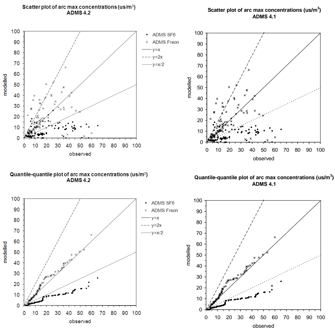
Figure 5 – Scatter plots and quantile-quantile plots of ADMS results against observed concentrations ( \mu\text{s/m}^3 ).
