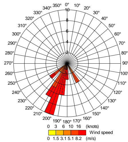
Figure 3 – Wind rose.
