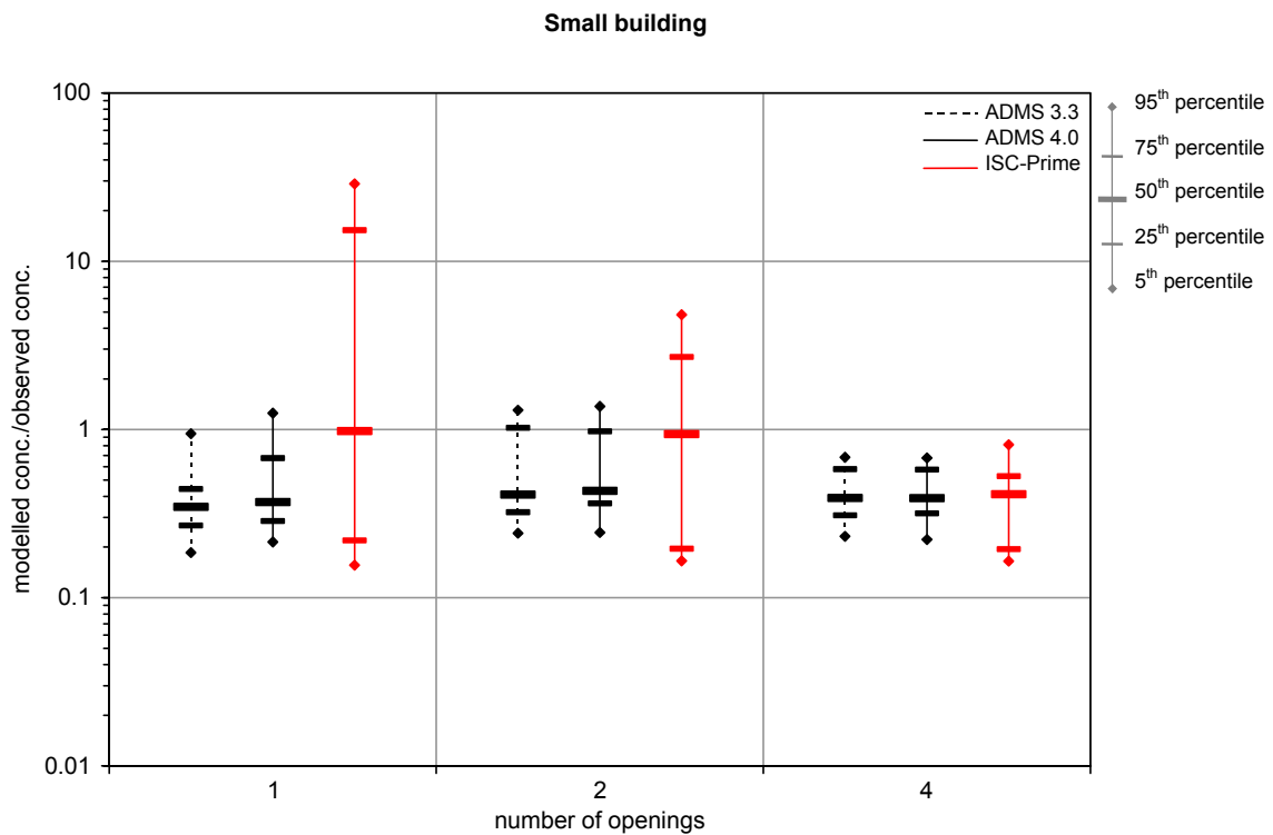
Figure 5 – Box and whisker plot of the results for the small building: roof openings.
