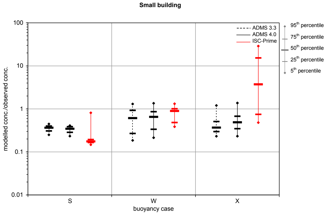
Figure 4 – Box and whisker plot of the results for the small building: buoyancy cases.
