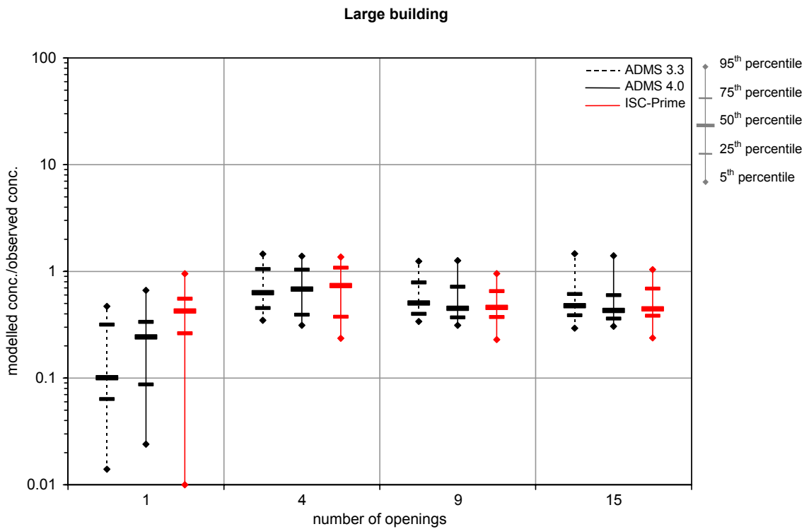
Figure 3 – Box and whisker plot of the results for the large building: roof openings.
